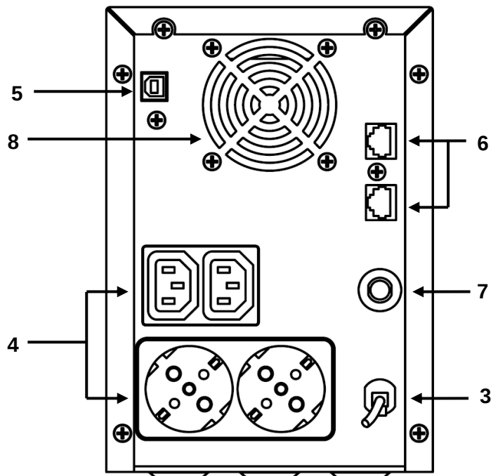
Rear view UPS NemoLCD 400
