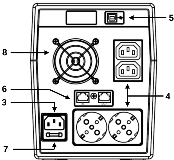
Rear view UPS NemoLCD 200-300
