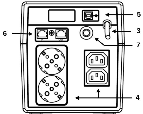
Rear view UPS NemoLCD 160
